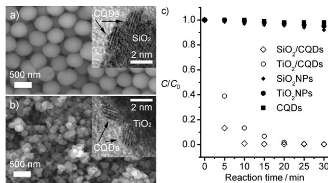
Figure 5. a,b) SEM image of photocatalysts for \text{SiO}_2/\text{CQDs} and \text{TiO}_2/\text{CQDs} ; insets show the corresponding HRTEM images; c) relationship between MB concentration and reaction time for different catalysts: \text{SiO}_2/\text{CQDs} , \text{TiO}_2/\text{CQDs} , \text{SiO}_2 NPs, \text{TiO}_2 NPs, and CQDs.
